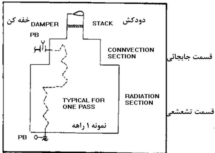
B) FIRED HEATER (BOX OR CYLINDRICAL TYPE) WITH COVECTION SECTION
